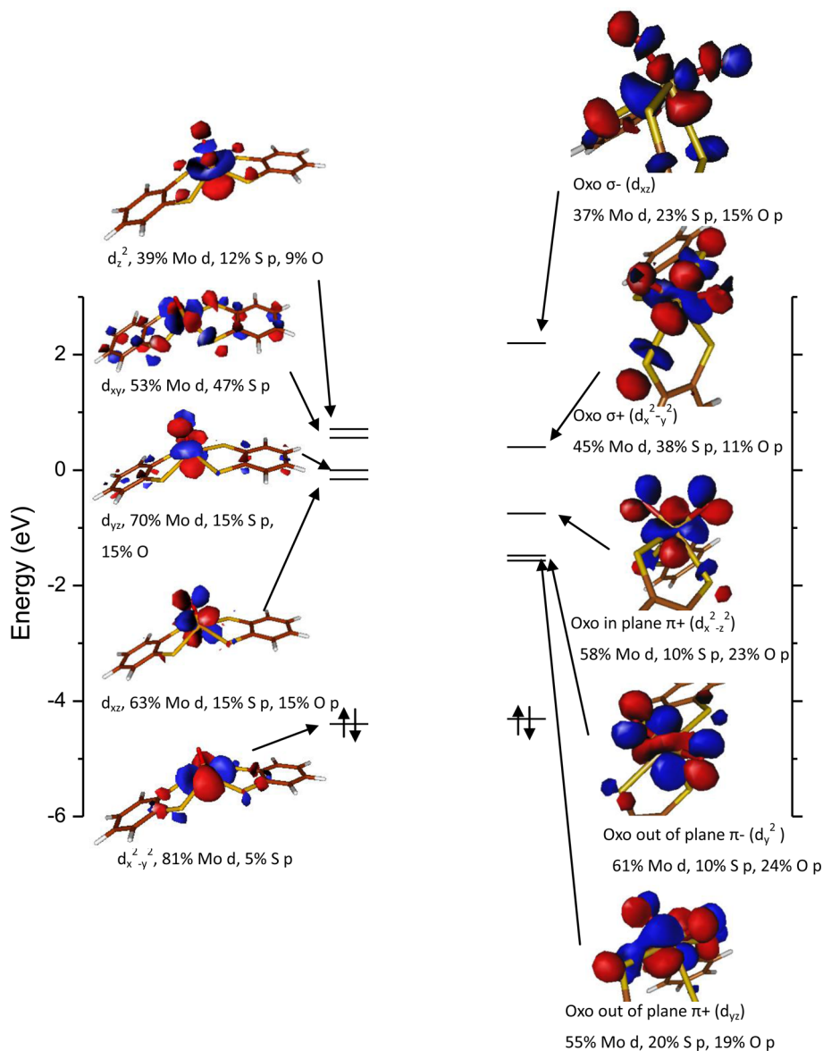
Figure 3. MO diagrams of [\text{Mo}^{\text{IV}}\text{O}(\text{bdt})_2]^{2-} (left) and [\text{Mo}^{\text{VI}}\text{O}_2(\text{bdt})_2]^{2-} (right). Selected atoms in [\text{Mo}^{\text{VI}}\text{O}_2(\text{bdt})_2]^{2-} have been removed for clarity.
